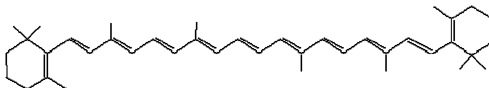
\beta -carotene (C 40 H 56 )
